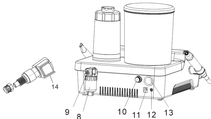
Figure 2 Rear Schematic Diagram
